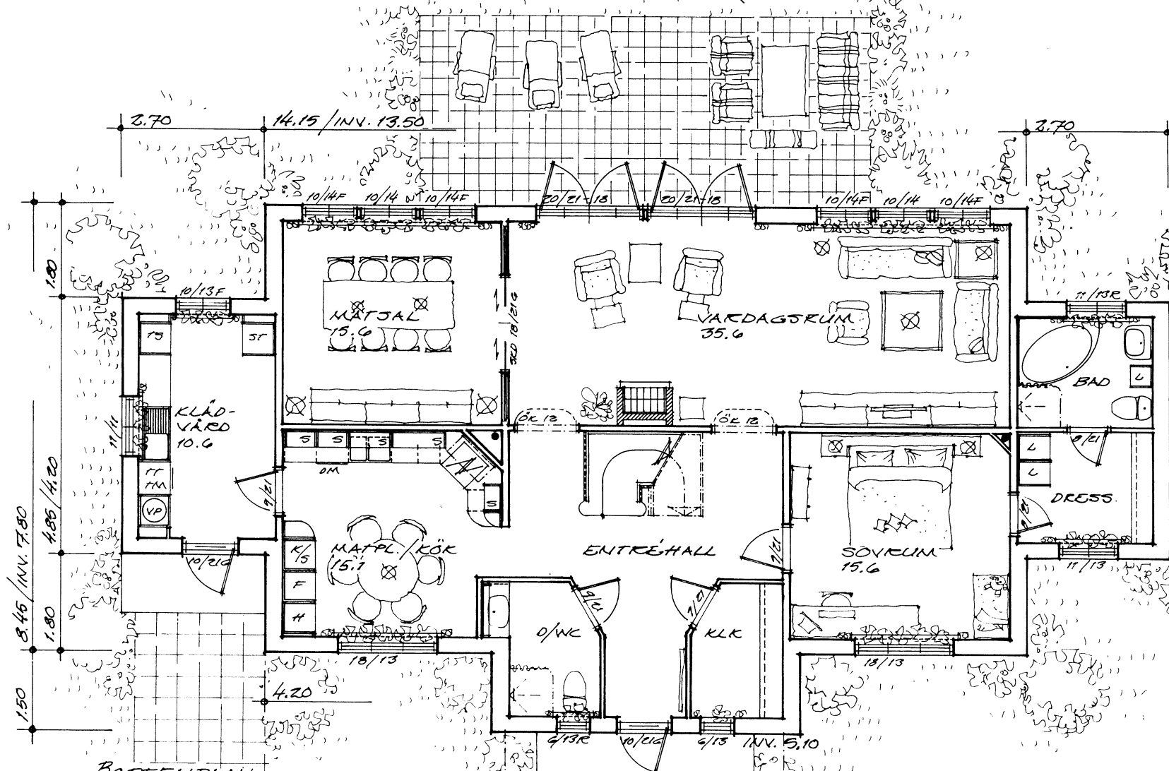
BOTTENPLAN BOAREÅ: 135.6 m 2
